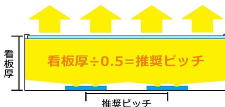
推奨看板厚 (50~150mm程度)
